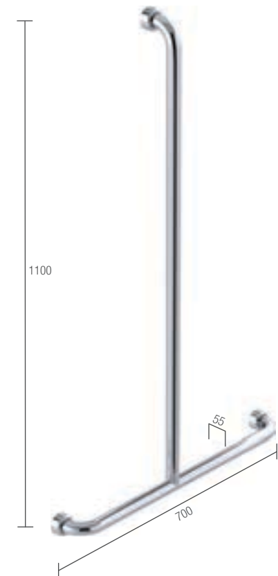
Drawn MF (Middle Fixed)
